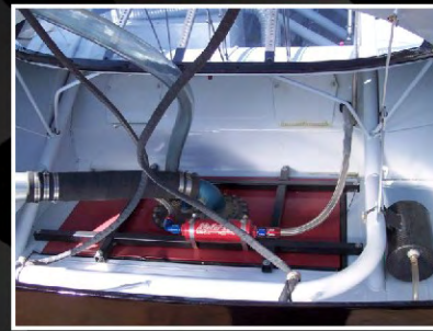
Fuel Cell
